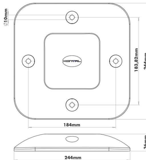
Figure 20 - Dimensions (mm)
