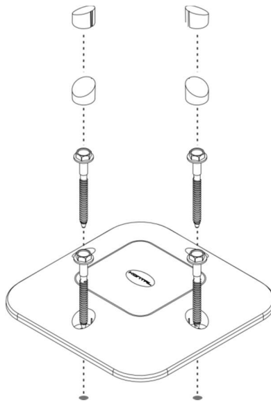
Figure 19 - The assembly will be completed by attaching screws and protective plastics.
