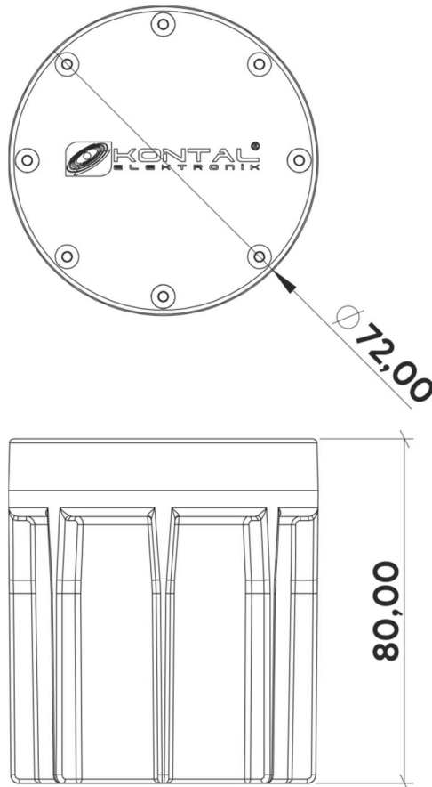
Figure 17- Dimensions(mm)
