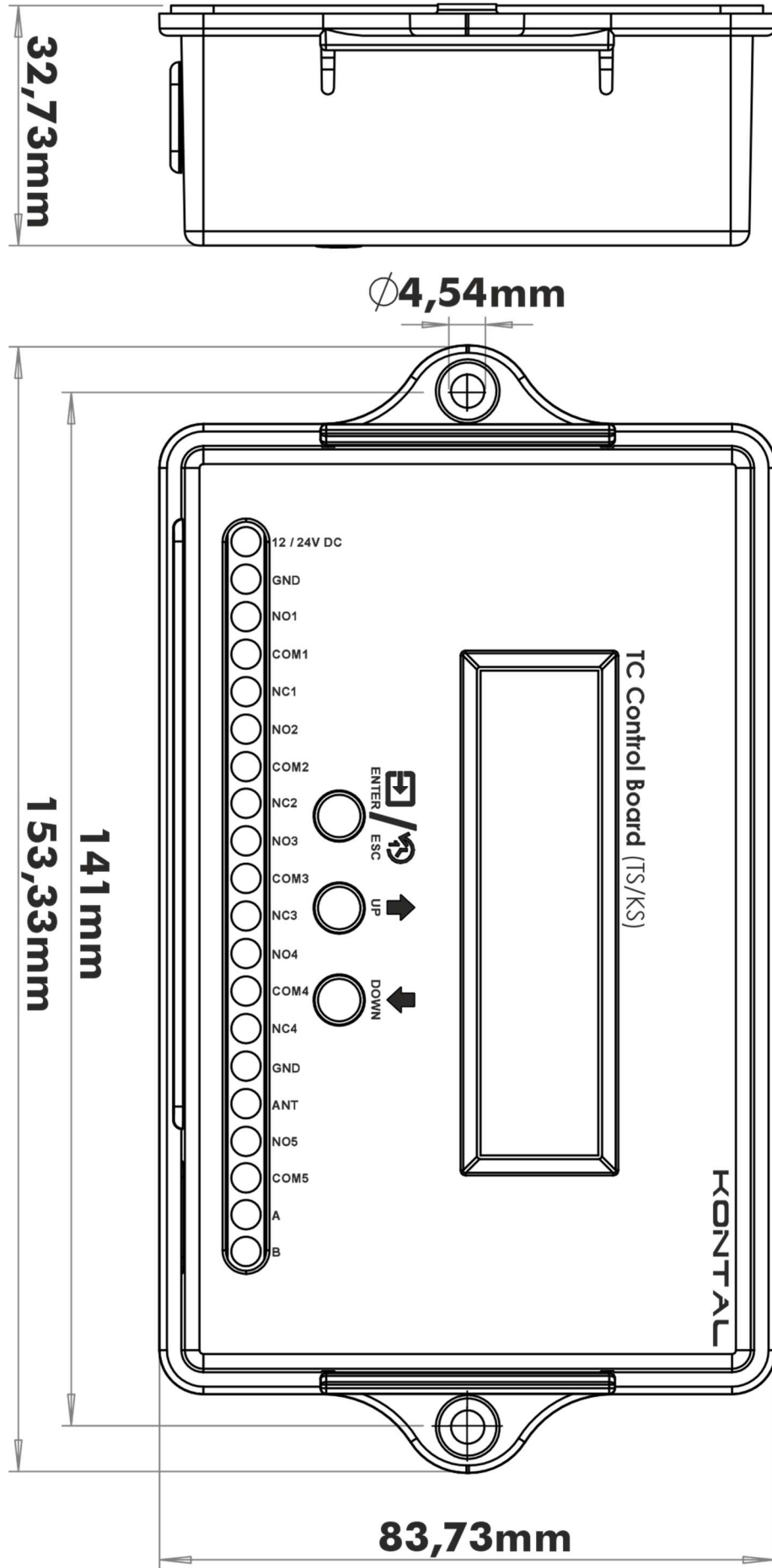
Figure 23 - Dimensions (mm)
