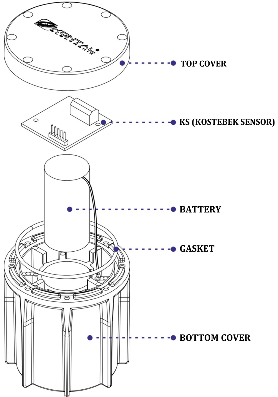
Figure 11 - KS board internal structure
