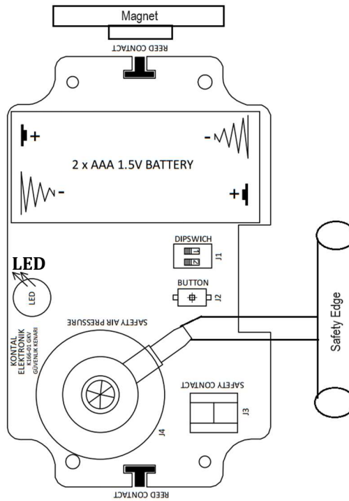
Figure 11 - GKV-B Connection Diagram
