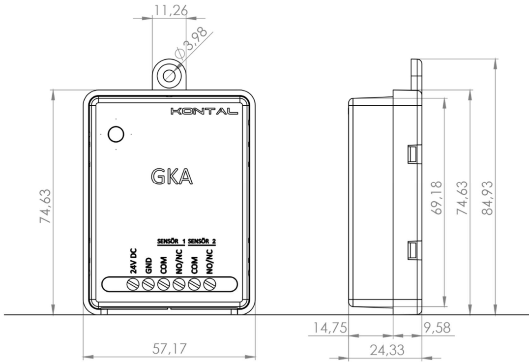
Figure 16 - GKA Dimensions
