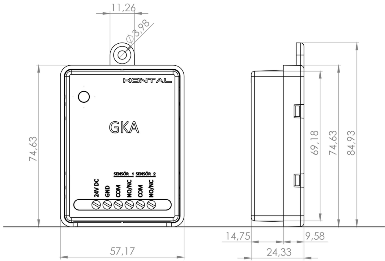
Figure 16 - GKA Dimensions (Unit = mm)
