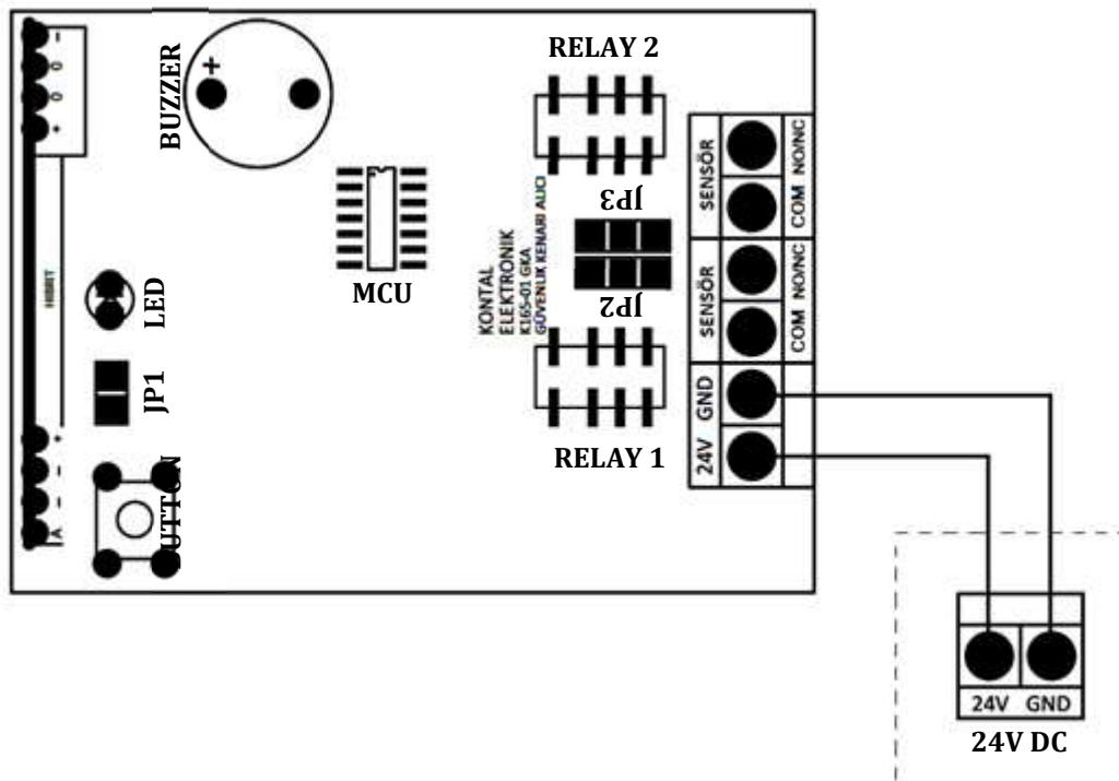
Figure 12 - GKA Connection Diagram
