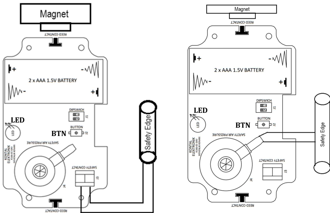
Figure 11 - GKV / GKV-B Connection Diagram
