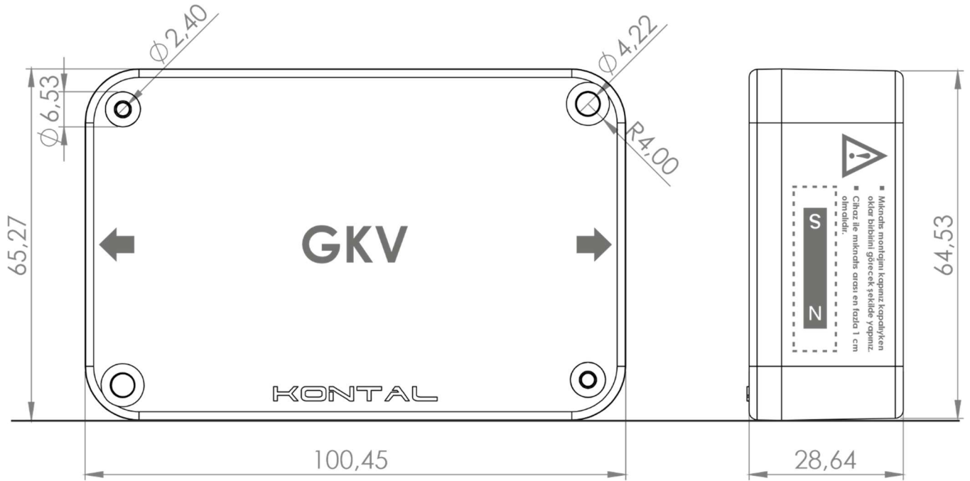
Figure 17 - GKV Dimensions (Unit = mm)
