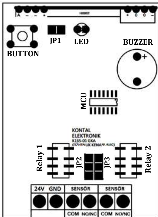
Figure 2 – Safety Edge Receiver (GKA)
