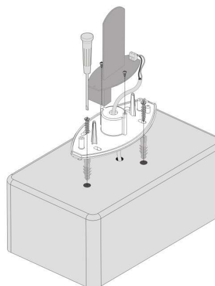
Figure 6.5 – FL Cable Connections and Surface Mounting
