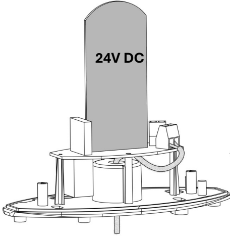
Figure 7.1 – Connecting the FL to 24V DC
