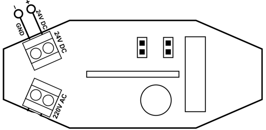
Figure 7.2 – Connecting the FL to 24V DC
