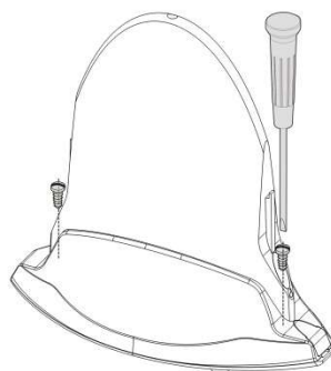
Figure 6.2 – Removal and Attachment of FL Screws
