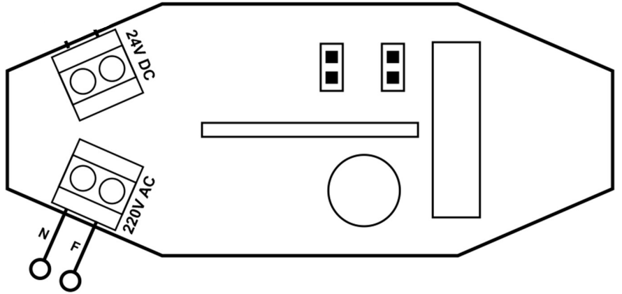
Figure 7.4 – Connecting the FL to 220V AC.
