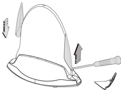
Figure 6.1 – Removal and Attachment of FL Side Brackets
