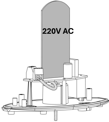
Figure 7.3 – Connecting the FL to 220V AC.
